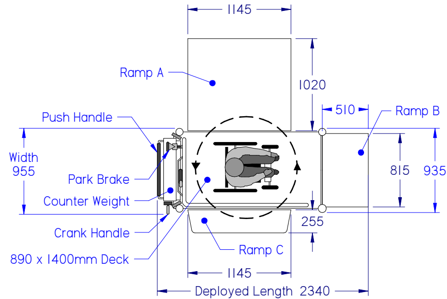
TOP ELEVATION - Standard Loading
