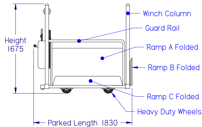
SIDE ELEVATION - Parked
