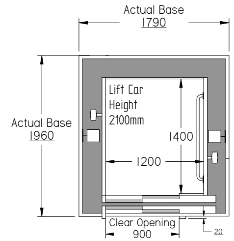
A MODEL PLAN Single Entry Car
