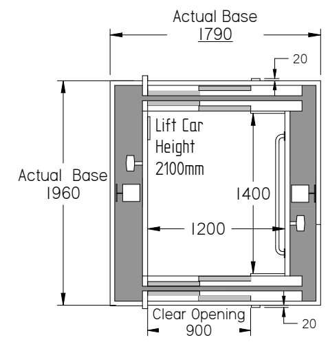
B MODEL PLAN Dual Entry Car
