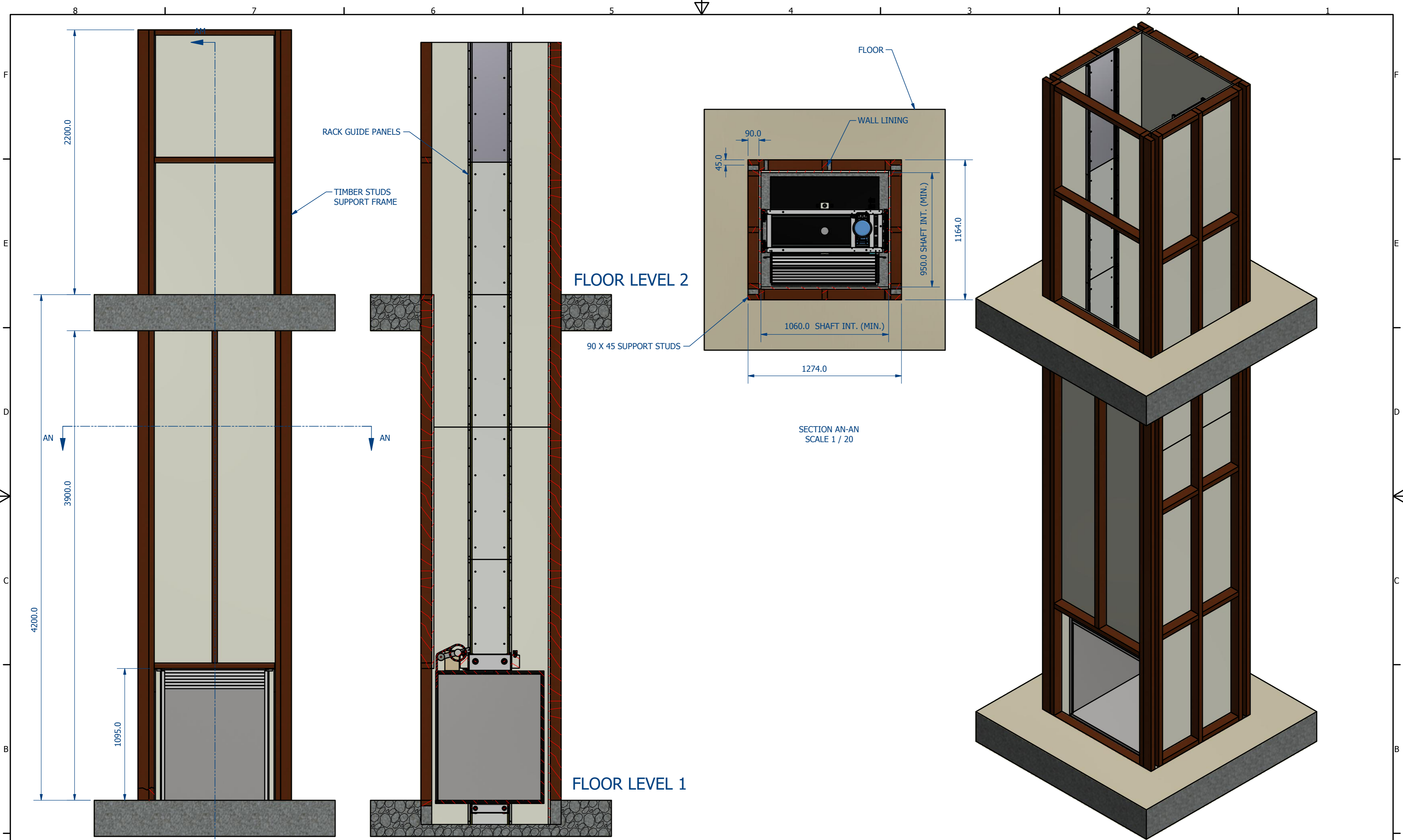
SECTION AM-AM SCALE 1 / 20
